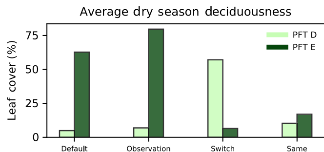
Fig. 7 Ecosystem Demography model 2 (ED2) simulated dry season deciduousness (from 2009 to 2014) for coexisting deciduous (PFT D) and evergreen (PFT E) plant functional types in a Costa Rican tropical dry forest under different parameterization for rooting depth allometry based on Xu et al. (2016). The dry season deciduousness is defined as the average ratio of active leaf area over maximum leaf area in April, the peak of dry season. Higher leaf cover means more evergreenness. In the 'Default' simulation, maximum rooting depth of PFT E was about twice the rooting depth of the PFT D. In the 'Observation' simulation, rooting depth parameters were assigned to the model's PFT E and PFT D based on the present study's measurements. In the 'Switch' simulation, the measured PFT D rooting depth was assigned to the model's PFT E, and vice versa . In the 'Same' simulation, PFT E and PFT D were both assigned the same rooting depth parameter, calculated as the mean value of the observation PFT E and PFT D parameters.
