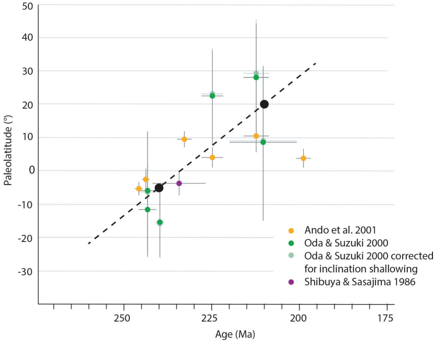
Fig. 7. Compilation of paleolatitudes derived from paleomagnetic data from the Inuyama cherts. The black dashed line represents the inferred paleolatitudinal motion of the Inuyama OPS (5°S at 240 Ma, 20°N at 215 Ma) used in the reconstruction.
